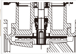
Pump casing design can ensure of the bearings' longevity & long time operation.
